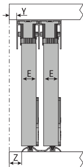
Riel AL Doble CX Triho Duplo CX Double Carrier Track CX
