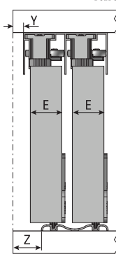
Riel AL Doble CX30 Triho Duplo CX30 Double Carrier Track CX30
